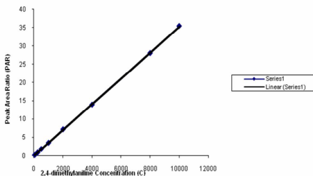
Figure 2. Calibration curve of 2,4-dimethylaniline in air
