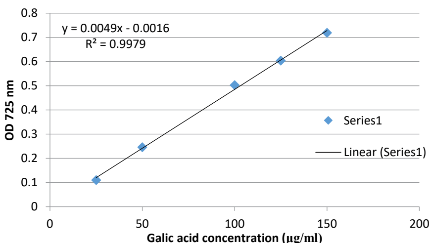
Figure 1. The Folin-Ciocalteu standard curve
