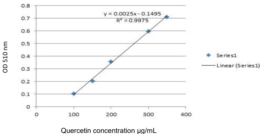
Figure 2. The Quercetin standard curve
